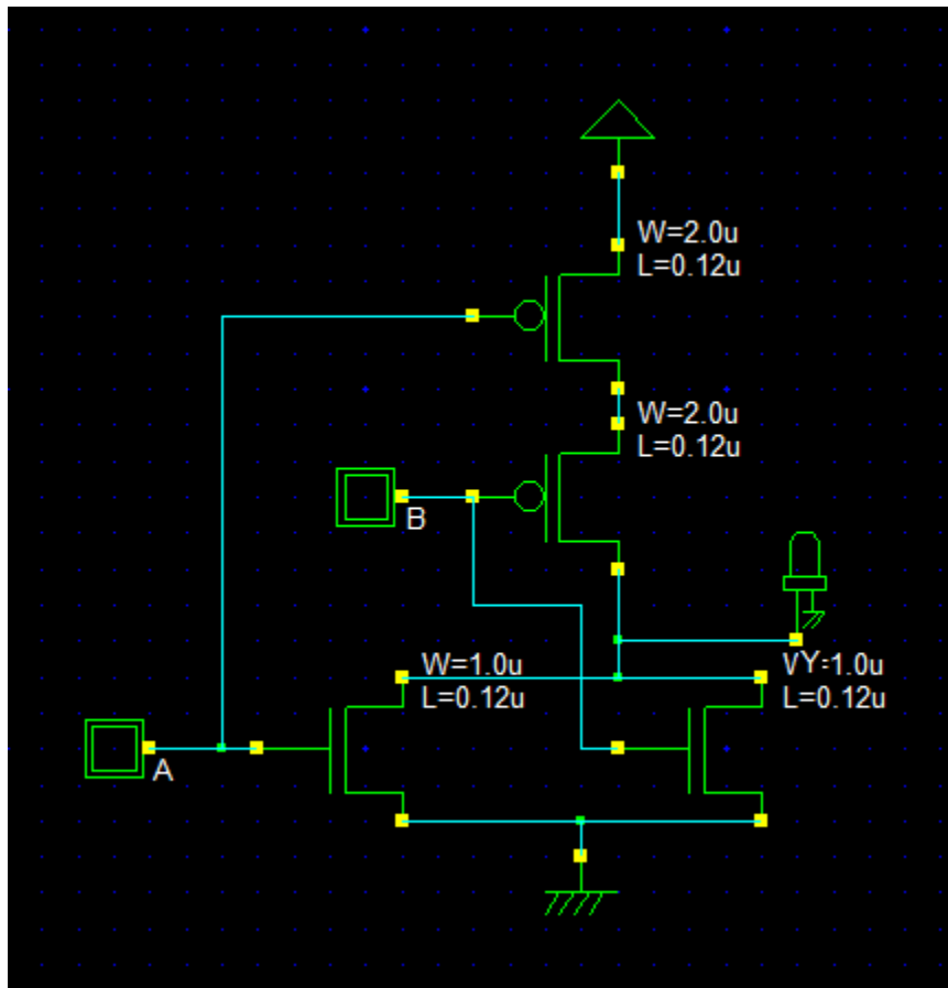
NOR Gate
